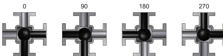
FLOW PLAN 13 4 Way L-Port - 360°
