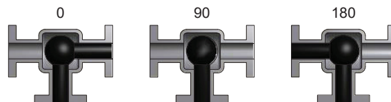
FLOW PLAN 18 3 Way L-Port - 180° (Bottom Entry)
