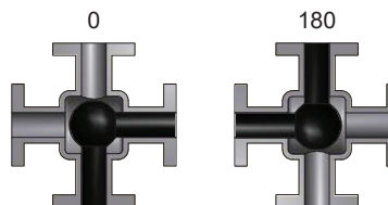
FLOW PLAN 12 4 Way L-Port - 180°
